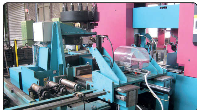
Sawing and machining line for rails (Luxembourg)
