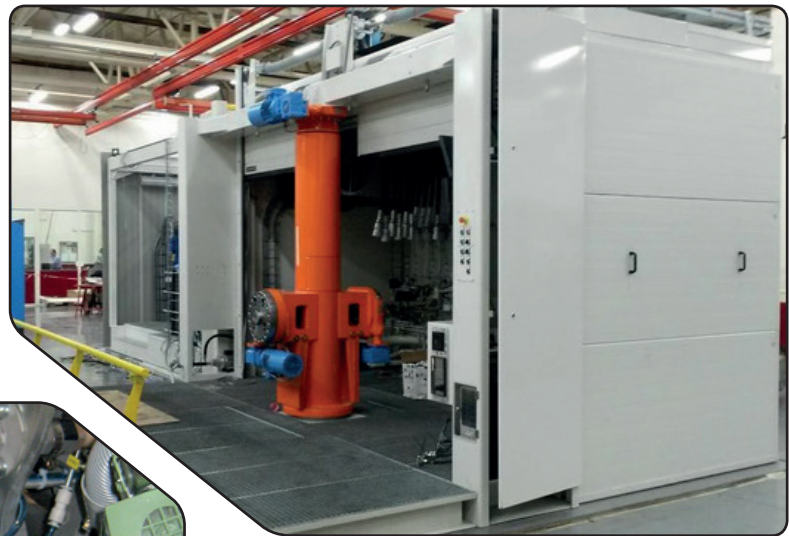
Testing units for hydraulic valves (Belgium)
