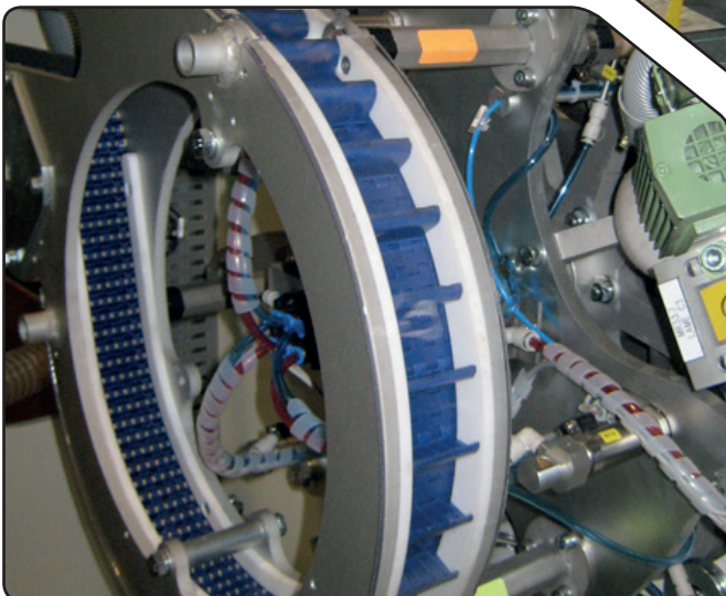
Chamfering unit for corks (Belgium)
